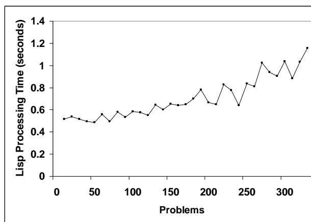
Figure 6. ACT-R Run Times for Blocks-World Problems
