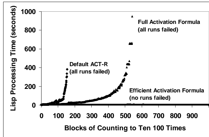
Figure 7. Comparison Long-Term Counting Runs with Different Parameters
