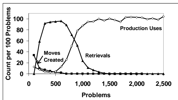
Figure 4. ACT-R Stages of learning
