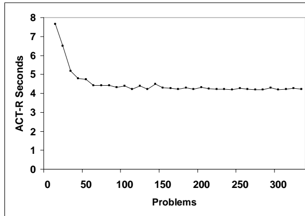
Figure 5. ACT-R Model Times for Blocks World Problems
