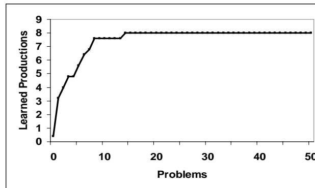
Figure 2: Productions Learned in Soar
